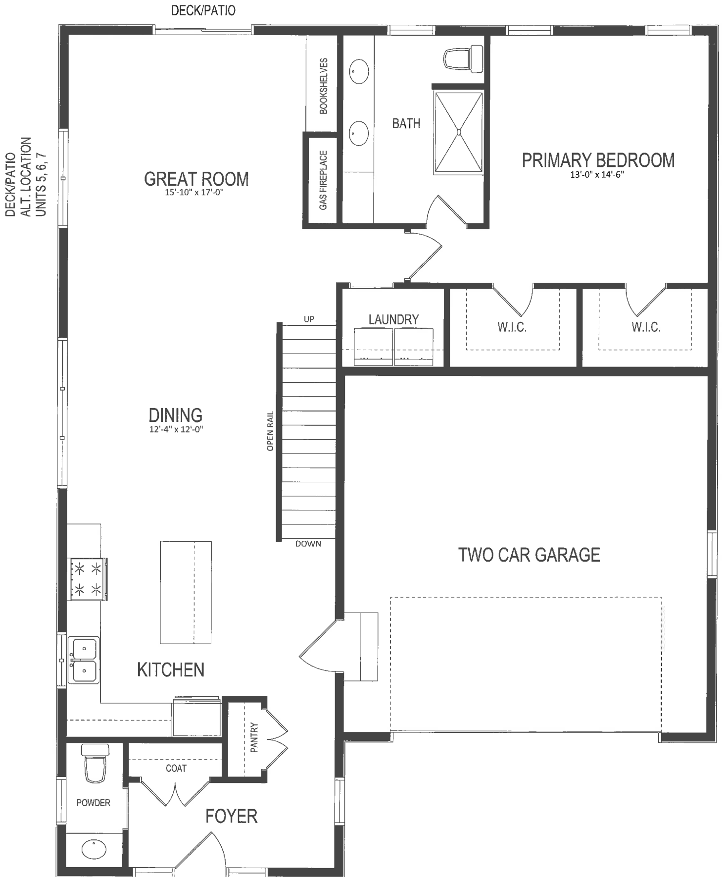
FIRST FLOOR PLAN 1,300 SF +/-
